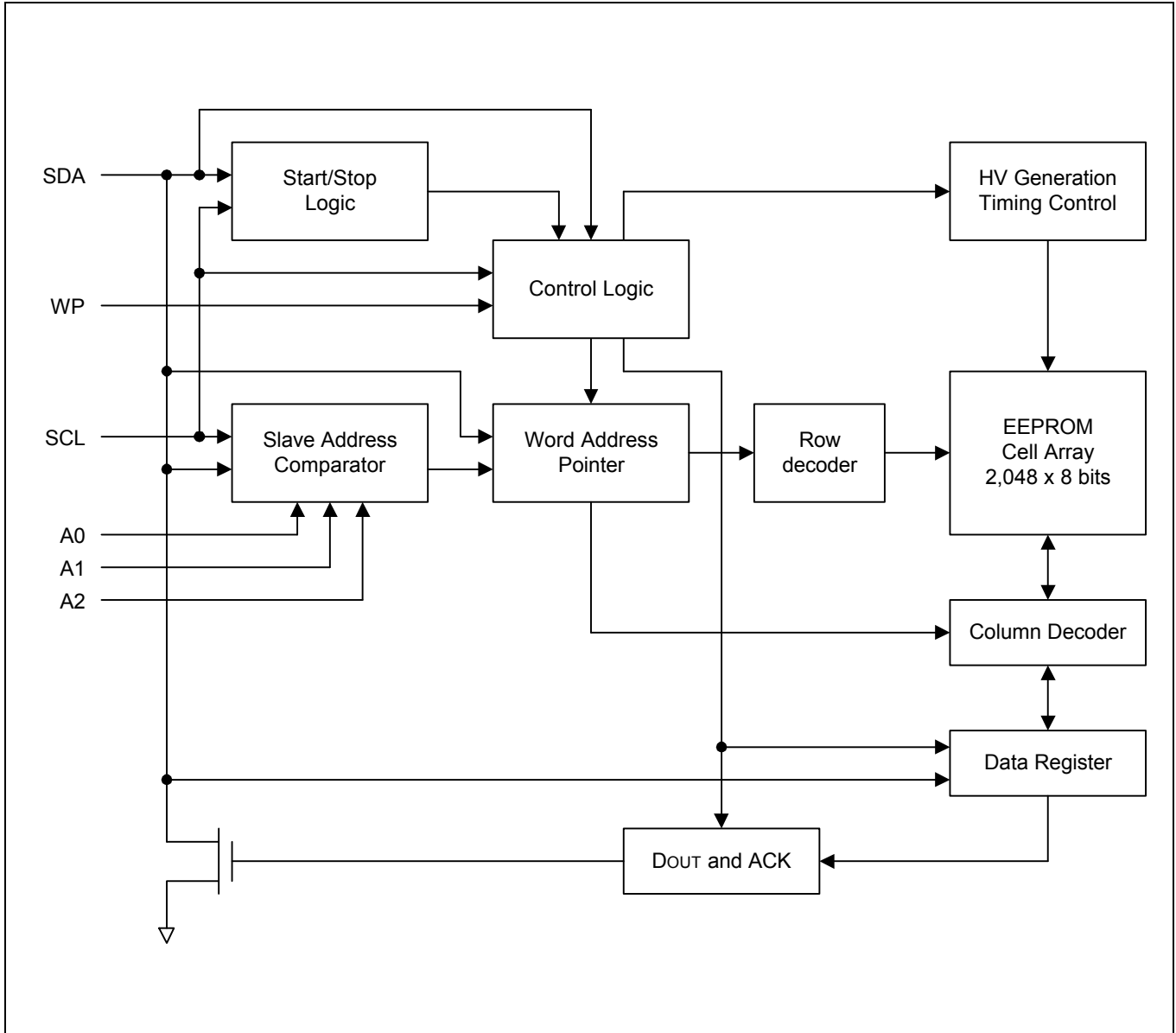
Figure 5-1. 24LC16 Block Diagram
