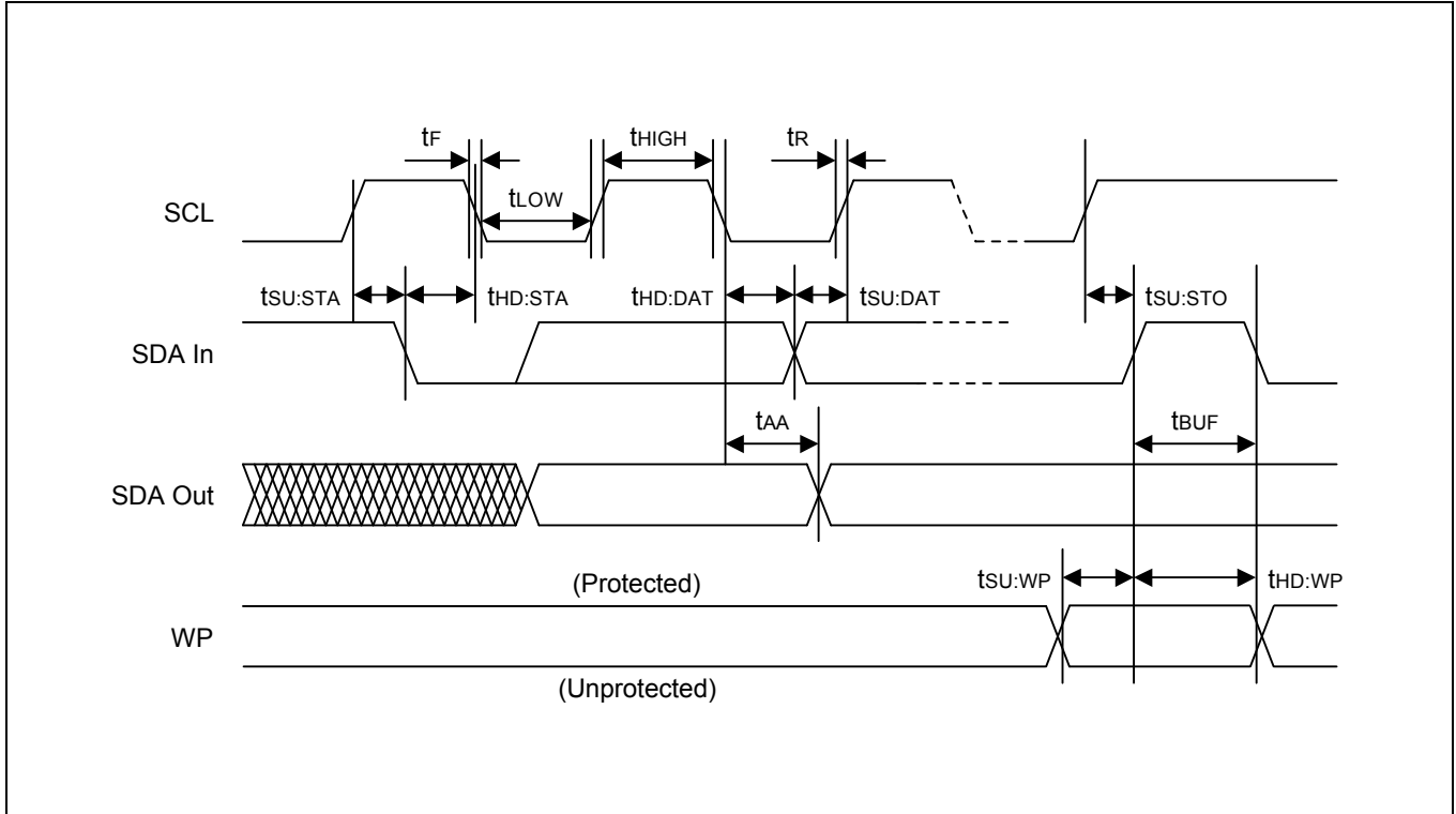
Figure 5-15. Timing Diagram for Bus Operations
