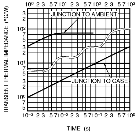
MAXIMUM TRANSIENT THERMAL IMPEDANCE CHARACTERISTICS
