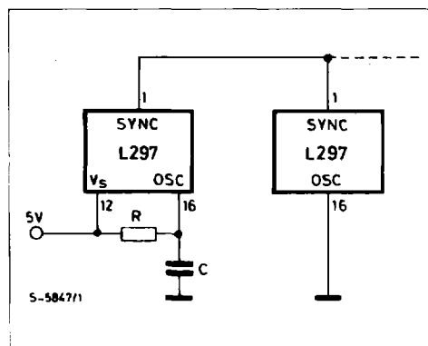
Figure 3 : Synchronising L297s
