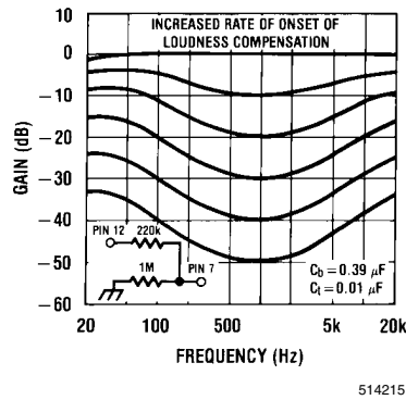
FIGURE 12. Loudness Compensated Volume Characteristic
