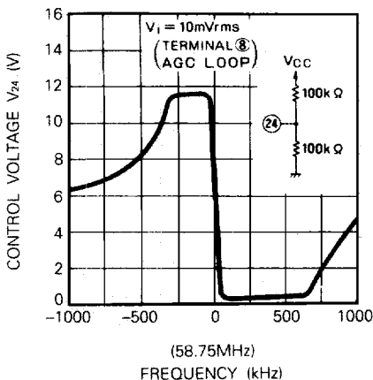
AFT WIDE BAND CHARACTERISTICS
