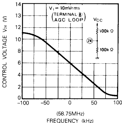
AFT NARROW BAND CHARACTERISTICS
