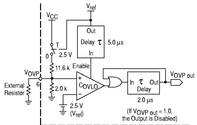
Figure 46. Overvoltage Protection
