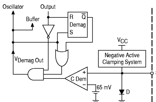
Figure 38. Demagnetization Block
