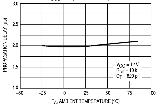
Figure 24. Propagation Delay ( V_{OVP} > 2.58\text{ V} to V_{out} Low) versus Temperature
