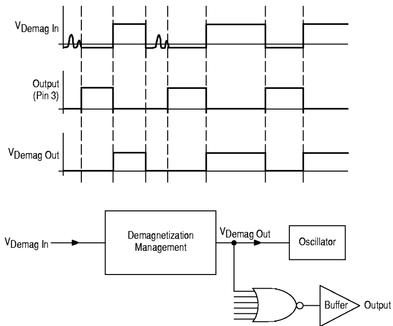
Figure 28. Demagnetization
