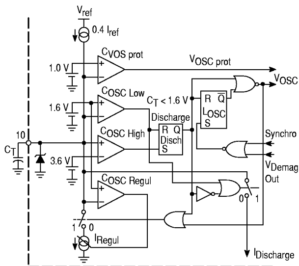
Figure 34. Oscillator
