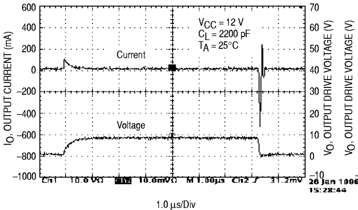
Figure 5. Output Waveform
