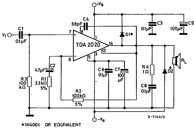
Fig. 16 - Application circuit with split power supply
