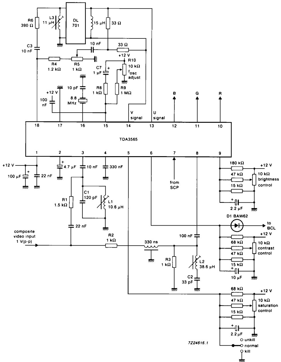
Fig. 5 Application diagram
