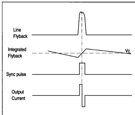
Figure 4 : Phase Comparator
