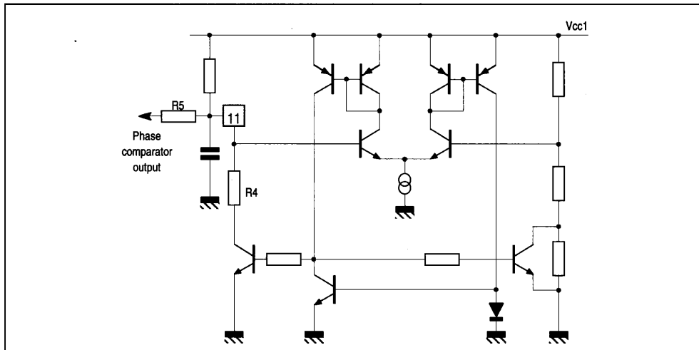
Figure 3 : Line Oscillator
