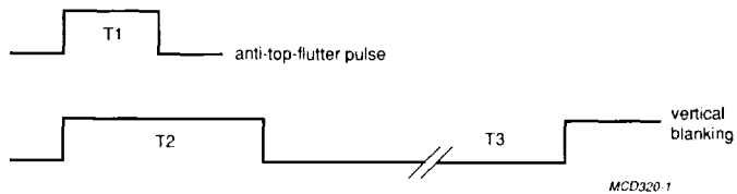
Fig.8 Anti-top-flutter pulse.
