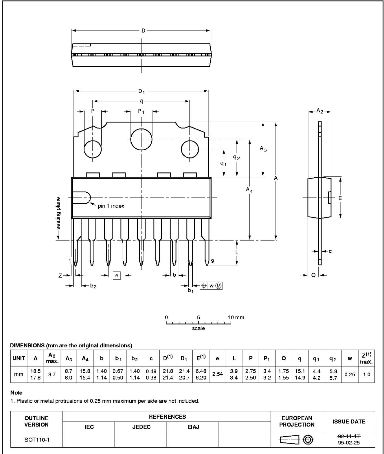
Fig 4. SIL9MPF package outline.
