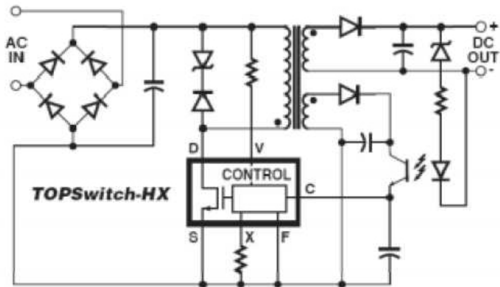
TOPSwitch-HX typical flyback application
