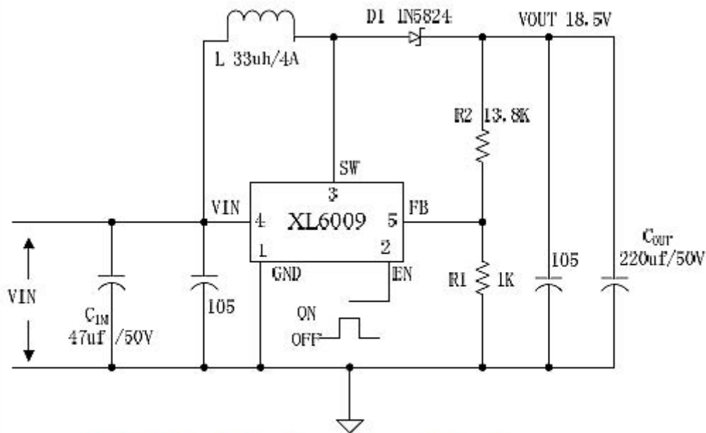
XL6009 Typical Application Circuit (Boost Converter)
