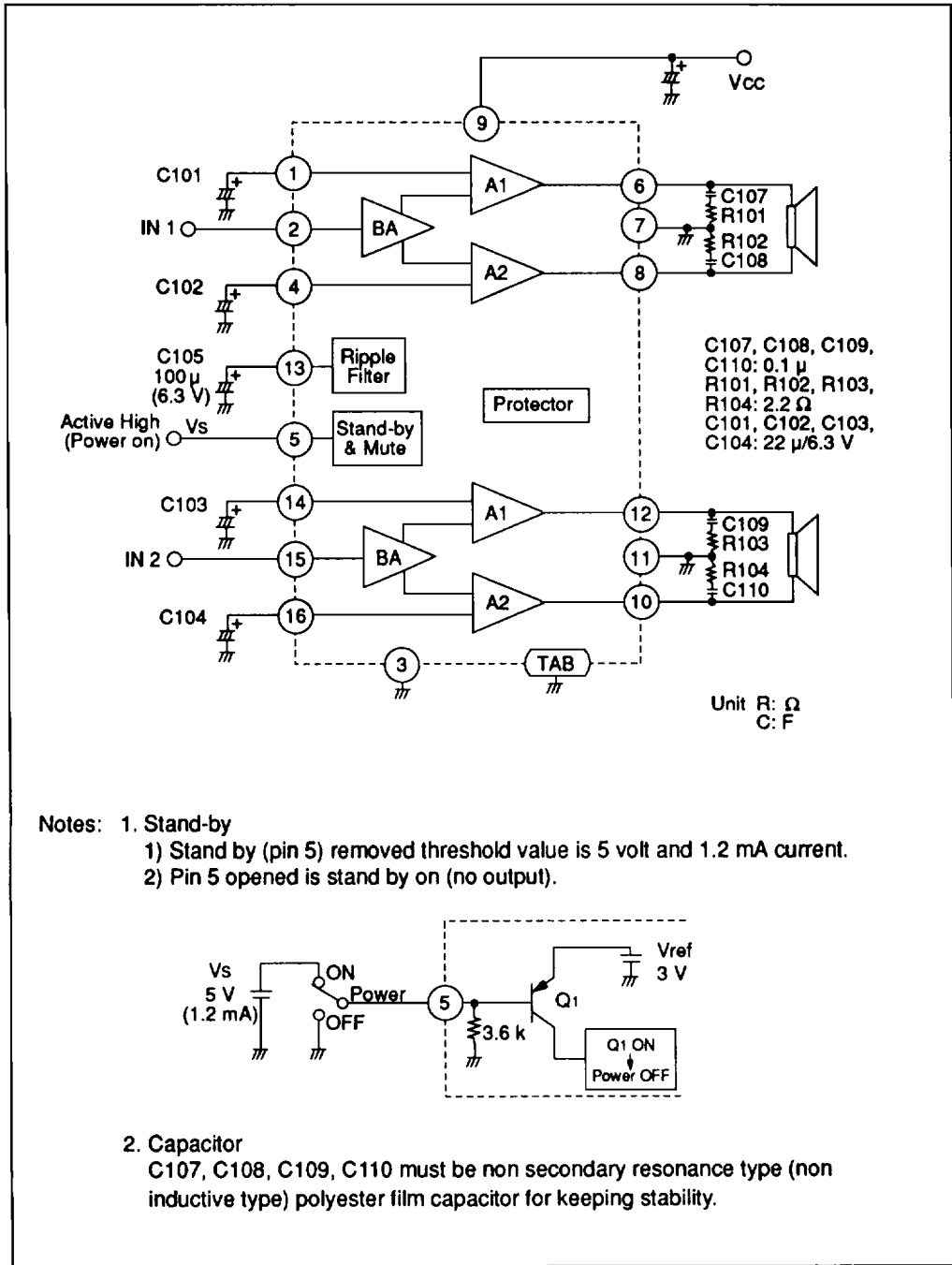
Figure 1 Block Diagram
