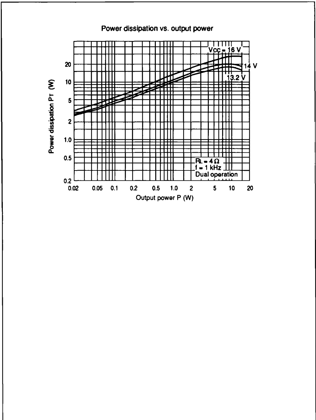
Figure 2 HA13130 Characteristic Curves (cont)
