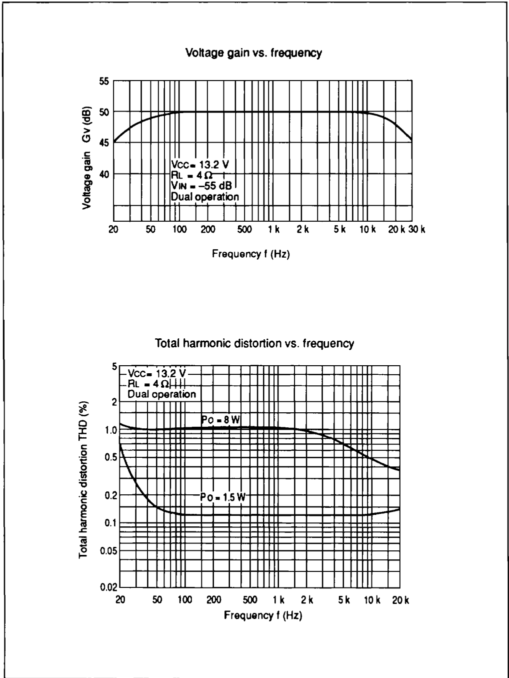
Figure 3 HA13127 Characteristic Curves (cont)
