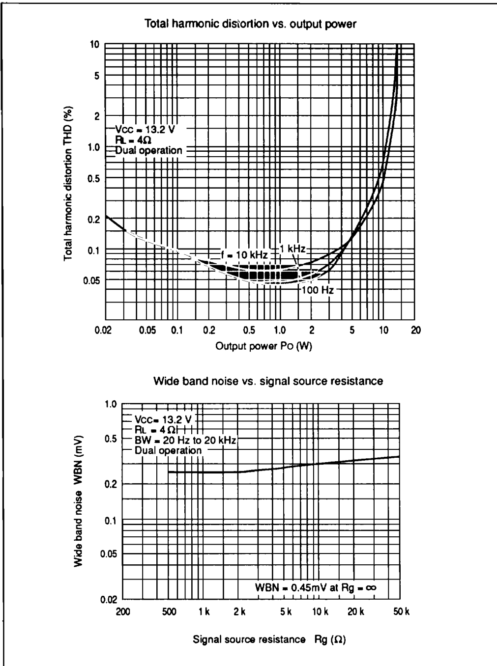
Figure 2 HA13130 Characteristic Curves (cont)
