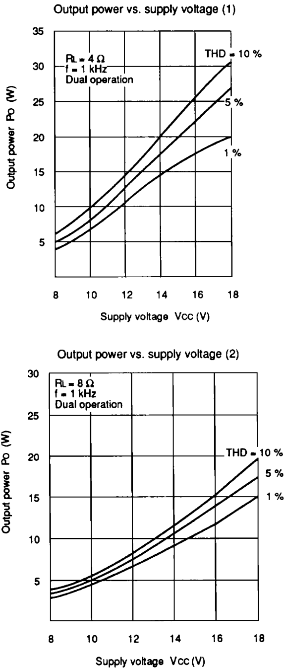
Figure 3 HA13128 Characteristic Curves (cont)
