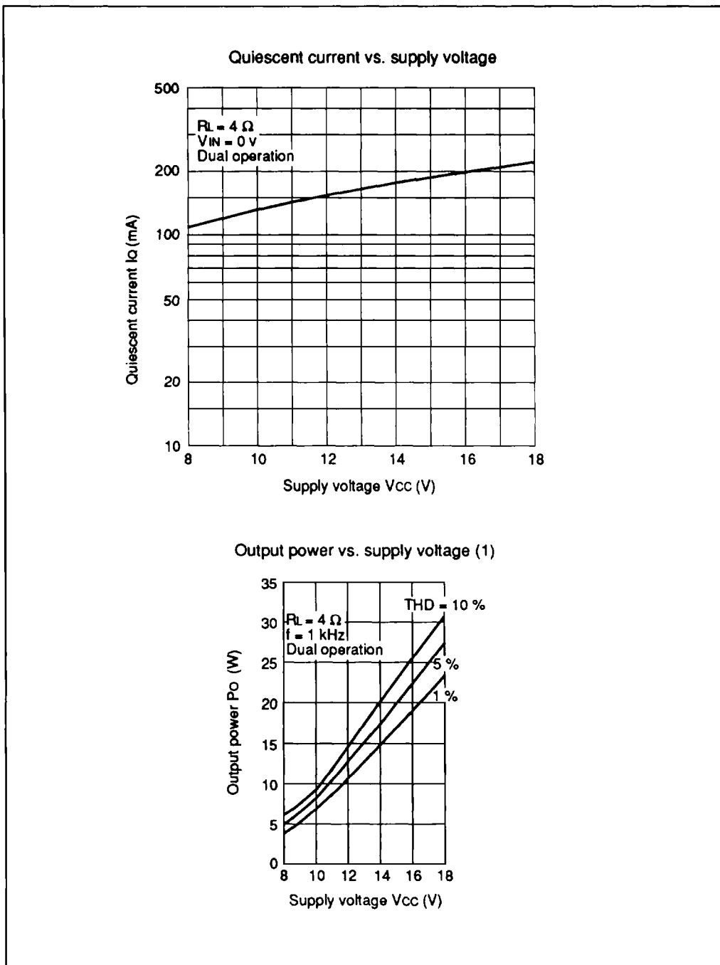
Figure 2 HA13135 Characteristic Curves
