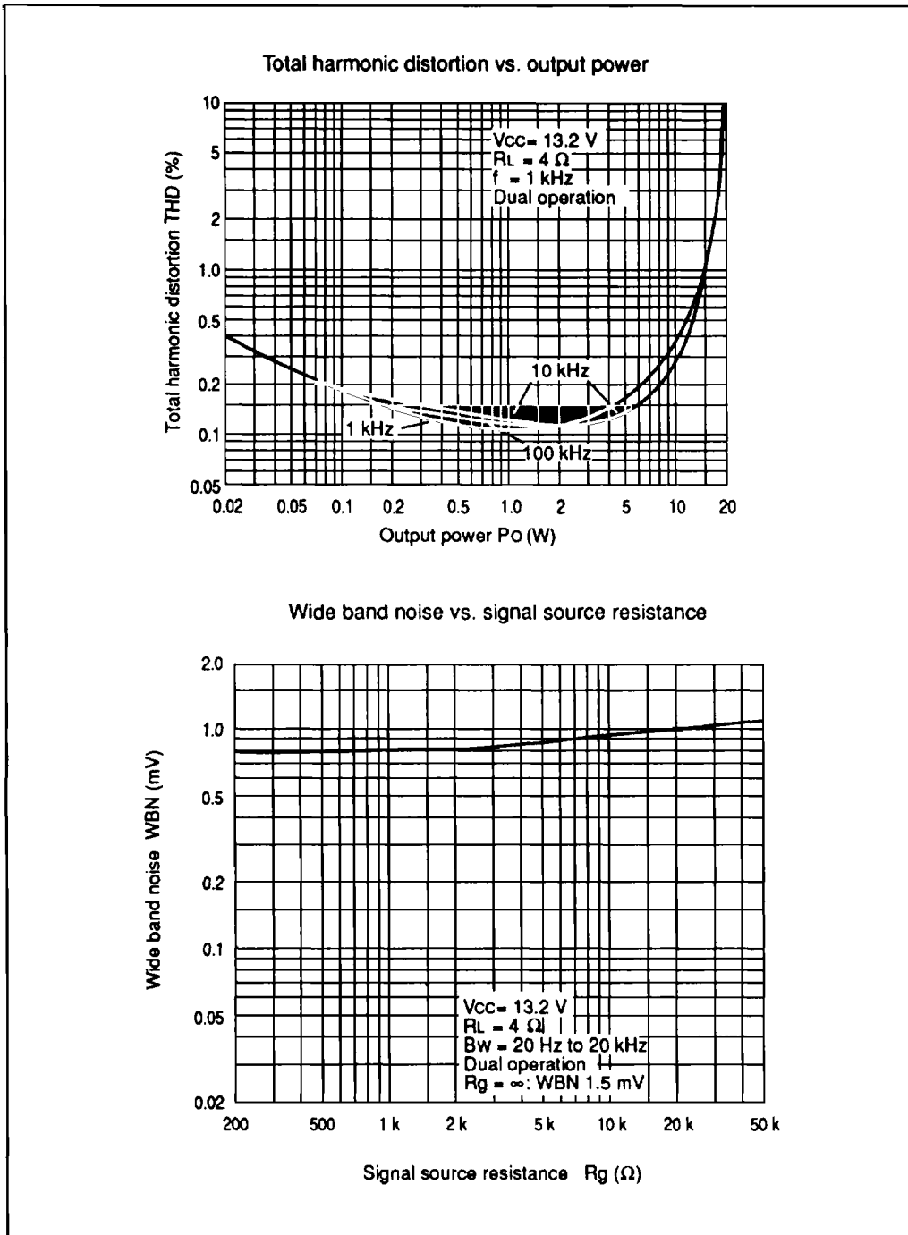
Figure 3 HA13128 Characteristic Curves (cont)
