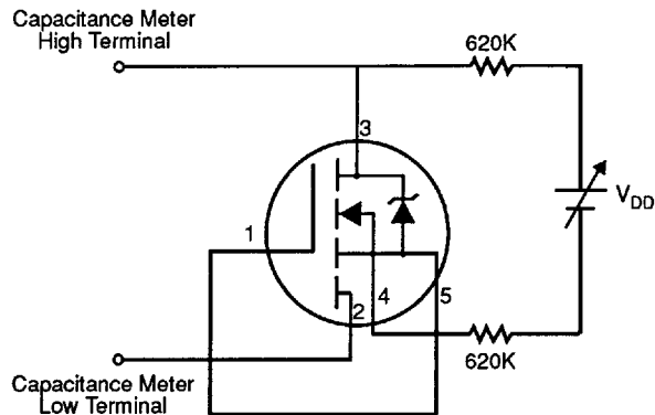
Fig 19. HEXSense Sensing Cell Output Capacitance Test Circuit
